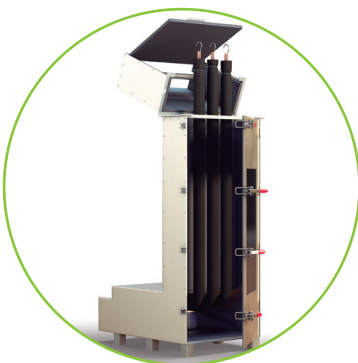
Insulated pipes are first inserted into a vertical pipe chase test chamber which mimics the actual pipe installation.
